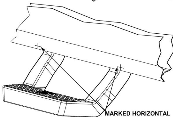
MARKED HORIZONTAL LINES 1/2" UP FROM BOTTOM OF PINCH WELD
